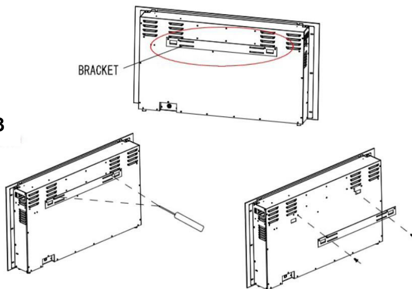
Wall Bracket Illustrated
